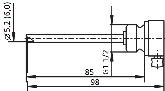
a) Dimensions of the temperature sensor pocket
