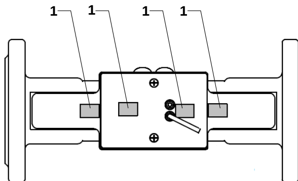
d) Flow sensor q_p = 15/25/40/60 \text{ m}^3/\text{h} sealing
