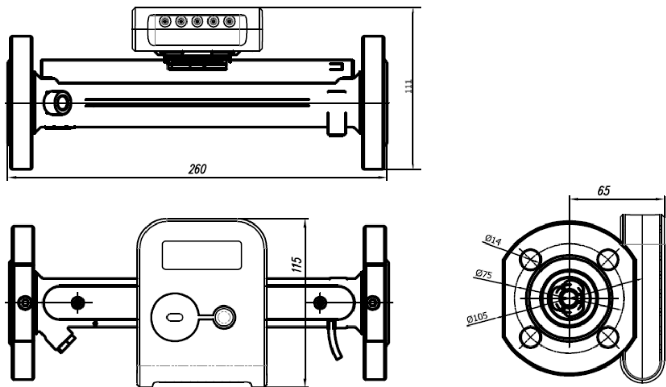
b) connection type: flanges DN25
