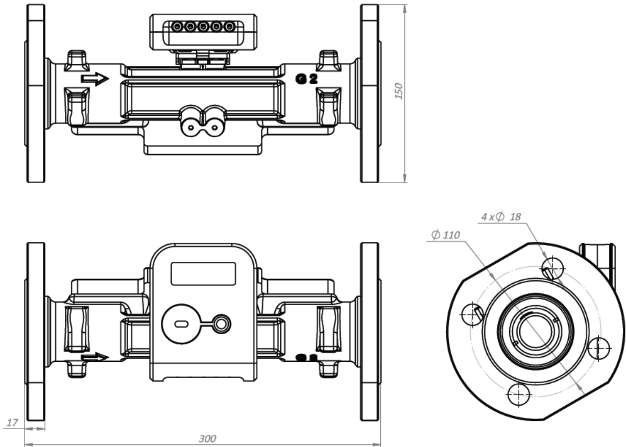
b) connection type: flanges DN40
