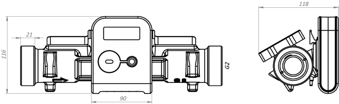
a) connection type: thread G2"
