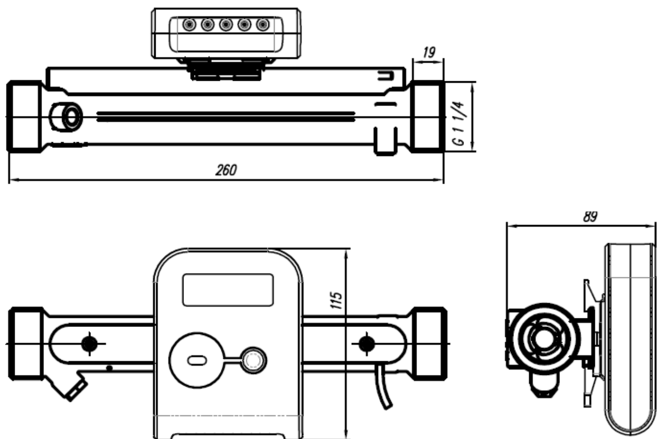
a) connection type: thread G1 1/4"
