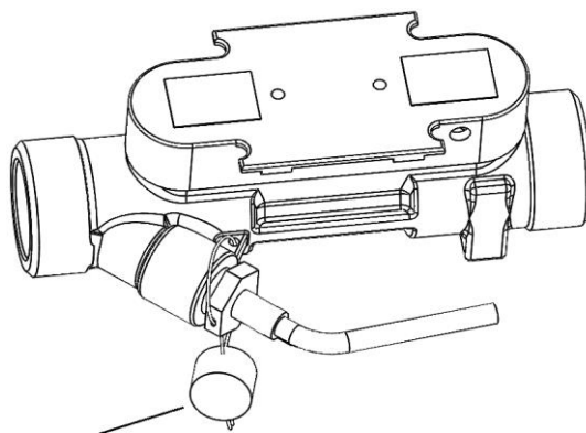
c) DS type temperature sensor installation in the flow sensor and sealing scheme.
