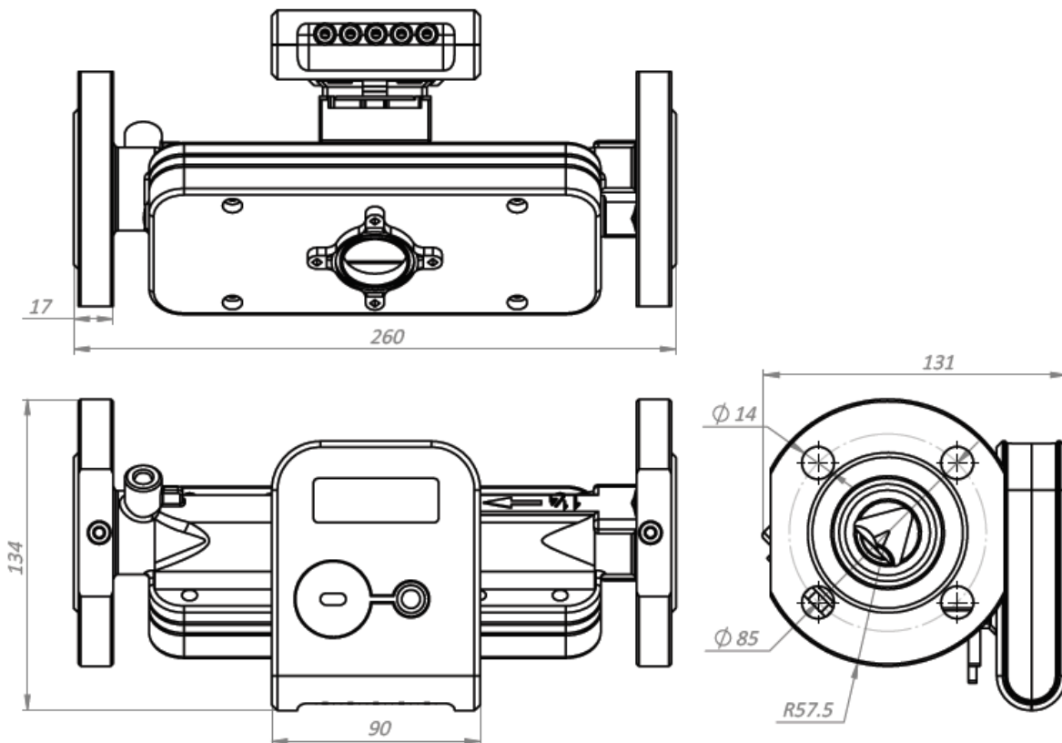
b) connection type: flanges DN25
