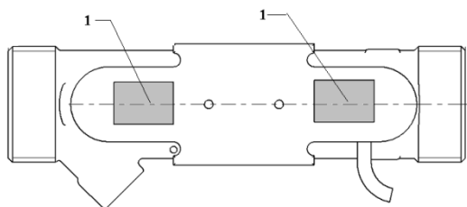
a) Flow sensor q_p = 0.6/1/1.5/2.5/3.5 \text{ m}^3/\text{h} sealing
