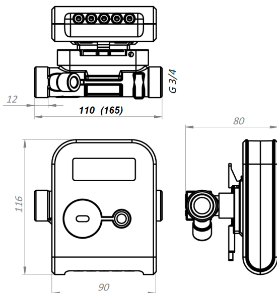
Fig. B2.1 Flow sensor q_p = 0.6/1.0/1.5 \text{ m}^3/\text{h} Length L=110 \text{ mm} ; connection type: thread G3/4"
