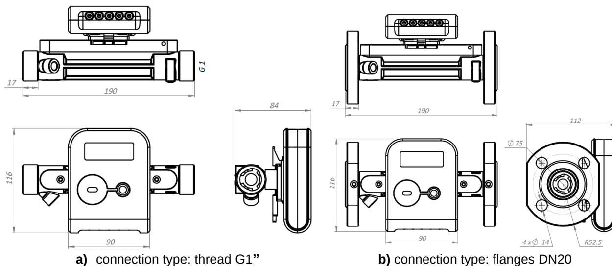
Fig. B2.3 Flow sensor q_p = 0.6/1/1.5/2.5 \text{ m}^3/\text{h} ; L=190 \text{ mm}
