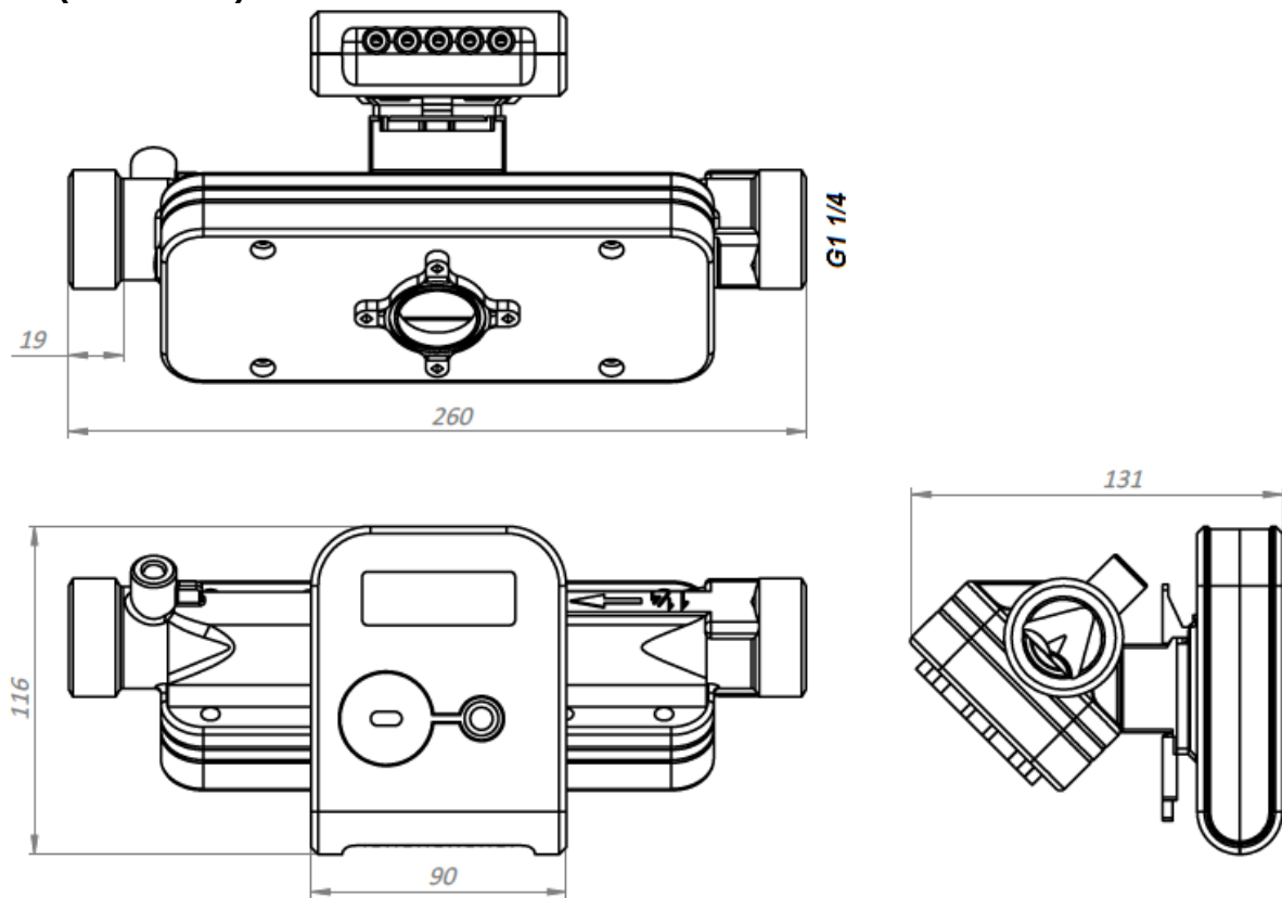
a) connection type: thread G1 1/4"
