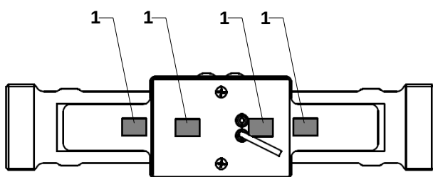
a) Flow sensor q_p = 0.6/1/1.5/2.5/3.5 \text{ m}^3/\text{h} sealing
