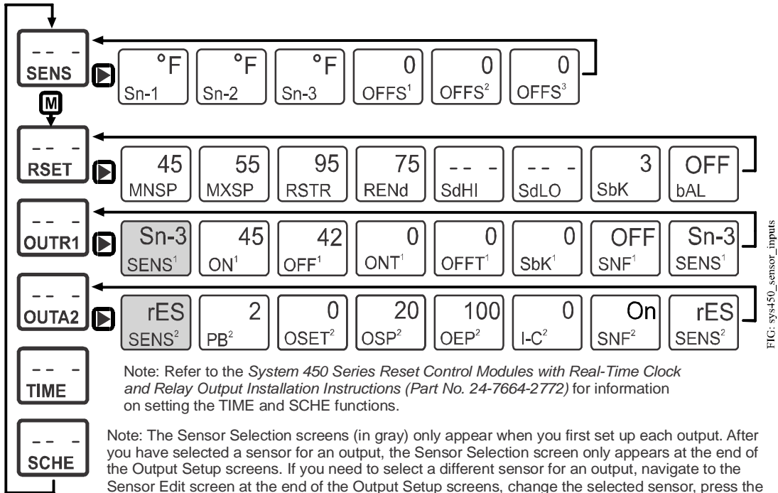
UI Screens for the Chilled Water Supply Reset Wiring Setup Example
