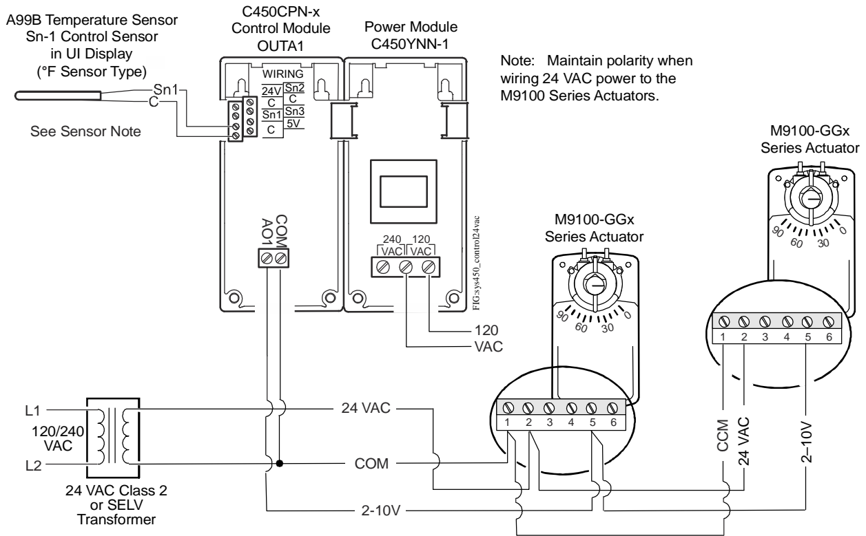
A C450CPN-x Control Module Powered by a C450YNN-1 Power Module Driving Up to Five M9100-GGA or M9100-GGC Actuators Wired in Parallel and Powered by a Dedicated 24 VAC External Transformer
