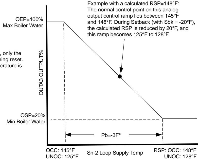
Control of Hot Water Supply to the Calculated RSP Temperature Using a Mixing Valve
