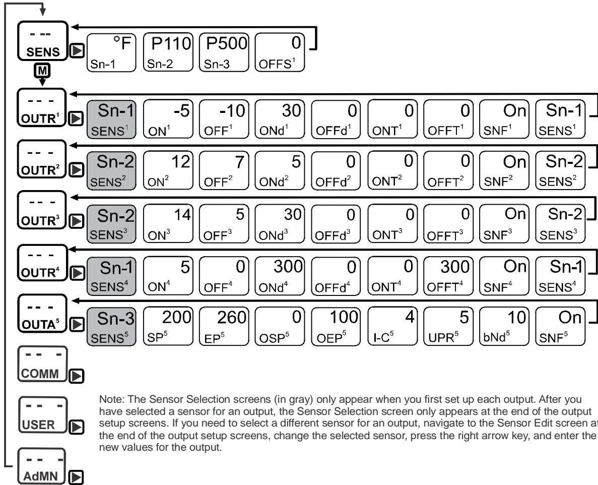
UI Screens for the Two-Stage Cooling Application with Remote Communications Example
