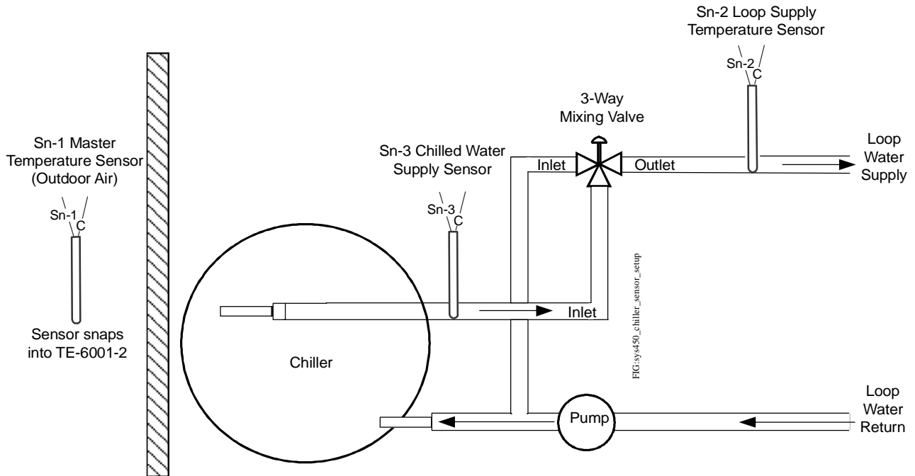
Chiller, Sensor, and Mixing Valve Setup
